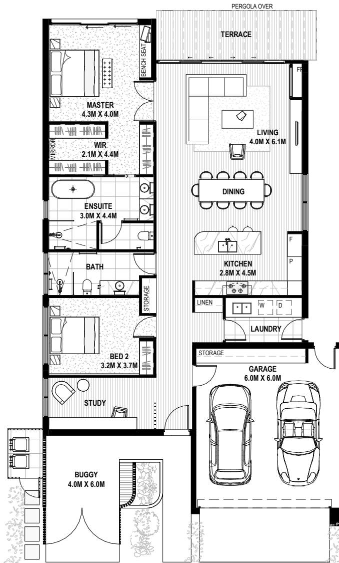
Ground Floor
